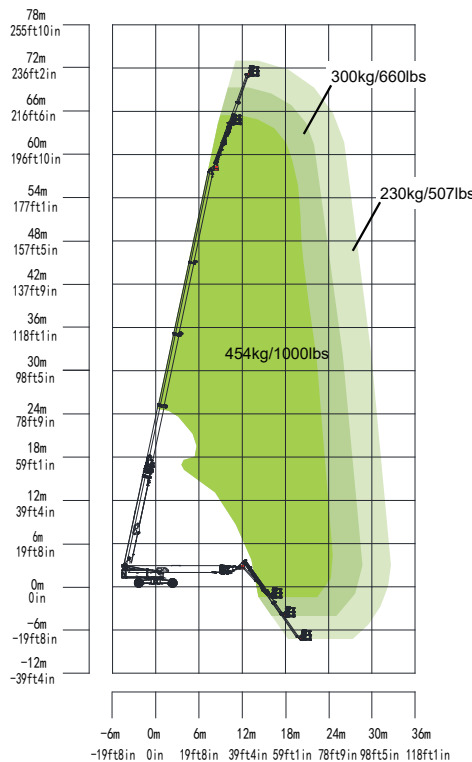
Range of Motion ZT72J-V
